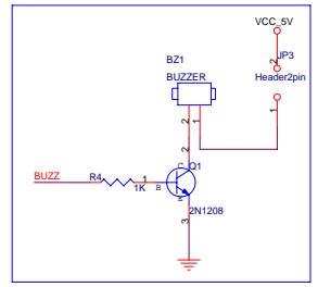
BUZZ
