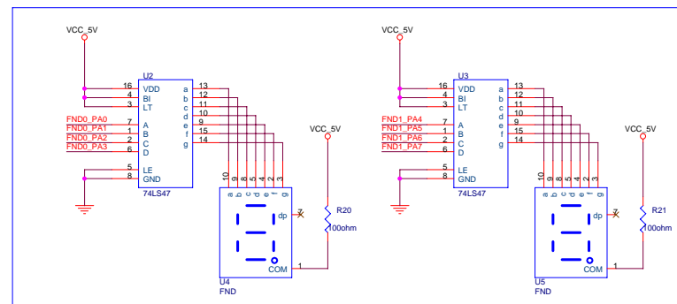
FND
