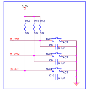
Ext Switch
