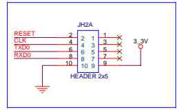
AVR Download Port
