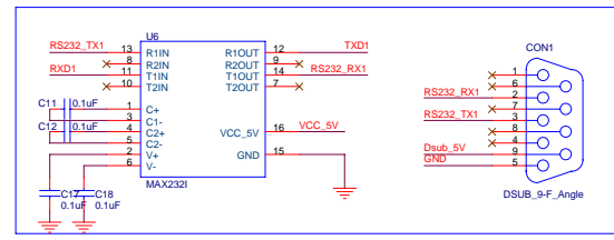
RS232
