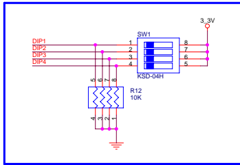
DIP Switch
