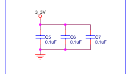
Bypass Condensor
