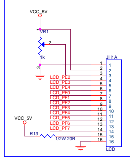
LCD Part
