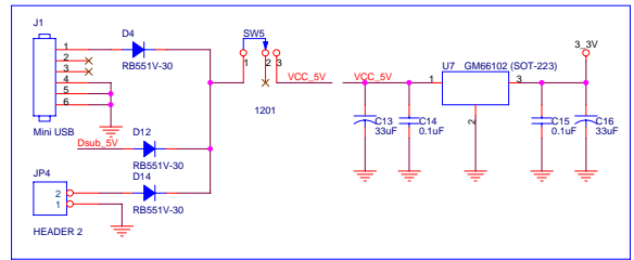
Power
